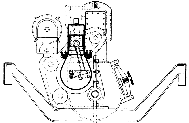
FRONT ELEVATION OF MOTOR AND SECTION THROUGH THE AIR-PUMP CYLINDER.
